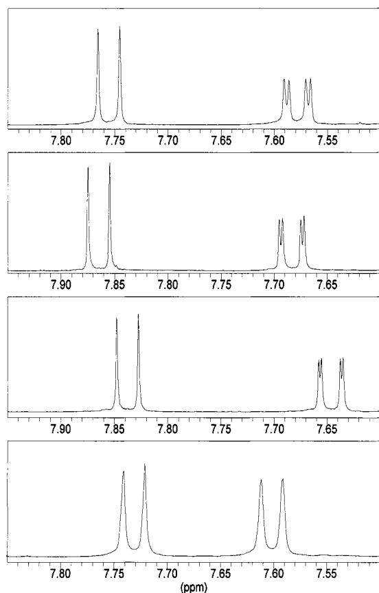
Figure 1. Expansion of ^1\text{H} -NMR spectrum of compound 1 in different solvents showing the signals assigned to H-6; anomer \beta : doublet; anomer \alpha : doublet of doublets due to through-space J_{\text{HF}} ; from top to bottom: \text{CDCl}_3 , [\text{D}_4]\text{methanol} , [\text{D}_6]\text{acetone} and [\text{D}_6]\text{DMSO}
