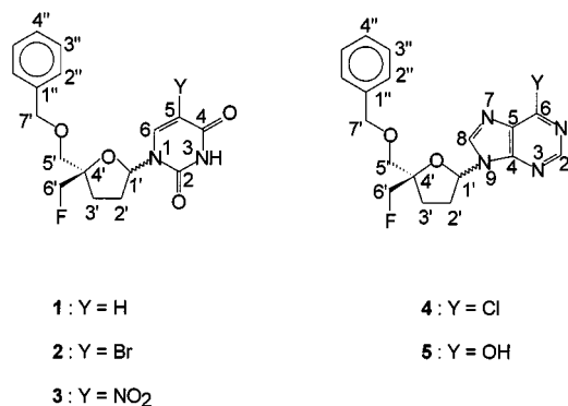
Scheme 1. Molecular formulae and structures of compounds 1–5
