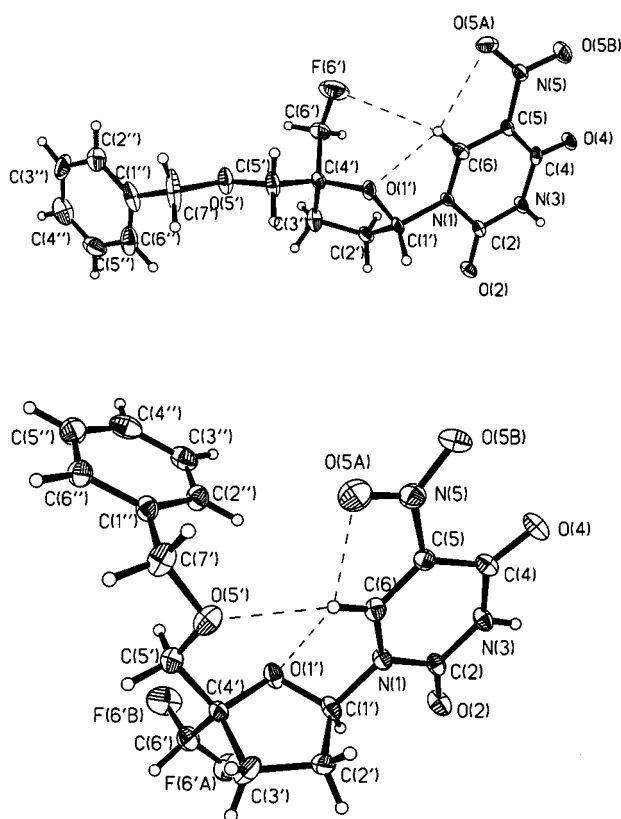
Figure 4. ORTEP view of 3a and 3b showing the atomic labelling scheme
