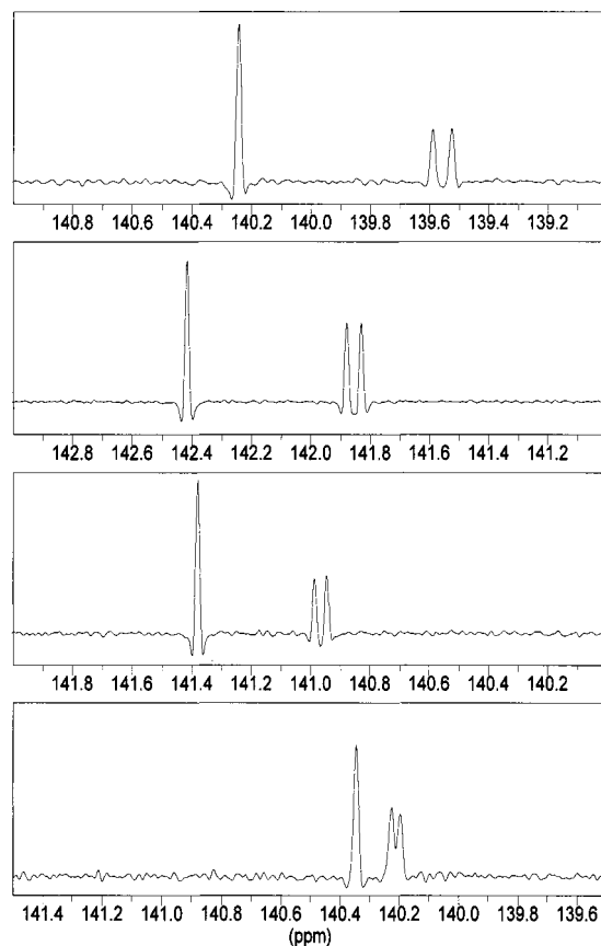
Figure 2. Expansion of ^{13}\text{C}\{^1\text{H}\} -NMR spectrum of compound 1 in different solvents showing the signals assigned to C-6; anomer \beta : singlet; anomer \alpha : doublet due to through-space J_{\text{CF}} ; from top to bottom: \text{CDCl}_3 , [\text{D}_4]\text{methanol} , [\text{D}_6]\text{acetone} and [\text{D}_6]\text{DMSO} ; the spectra are resolution-enhanced by gaussian multiplication prior to Fourier transform
