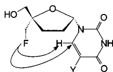
Scheme 2. Through-space {}^7J_{HF} and {}^6J_{CF} couplings constants
