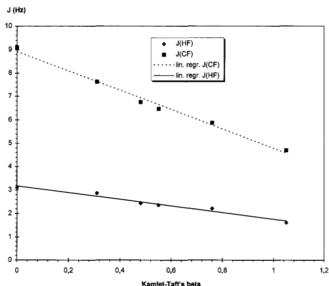
Figure 3. Plot of experimental through-space spin-spin coupling constants of compound 3 vs. Kamlet-Taft's parameter \beta
