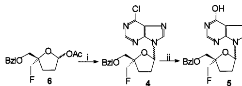
Scheme 4. Reagents and conditions: (i) 6-chloro-9-(trimethylsilyl)purine ( Y = Cl ); CH_2Cl_2 ; TMSOTf; room temp.; (ii) NaOH, CH_3OH , H_2O ; \Delta T
