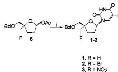
Scheme 3. Reagents and conditions: (i) 2,4-bis(trimethylsilyloxy)uracil ( R = H ), 5-bromo-2,4-bis(trimethylsilyloxy)uracil ( R = Br ), 5-nitro-2,4-bis(trimethylsilyloxy)uracil ( R = NO_2 ); (CH_2Cl)_2 ; TMSOTf; room temp.
